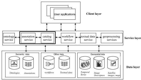
Figure 1: WebMAPS 3-layer Architecture
