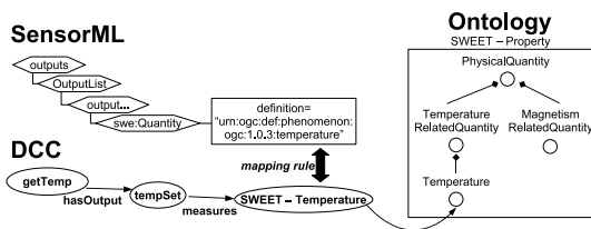
Figure 2: Mapping SML to DCC Metadata.
