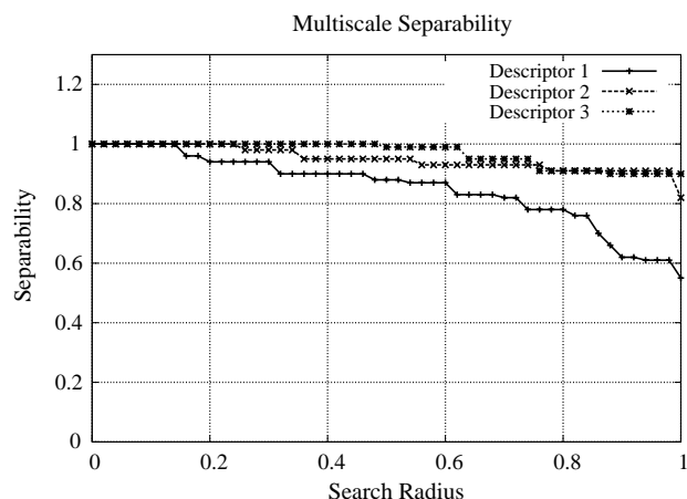
Fig. 11. Multiscale separability: as higher is the curve, as better is the descriptor.
