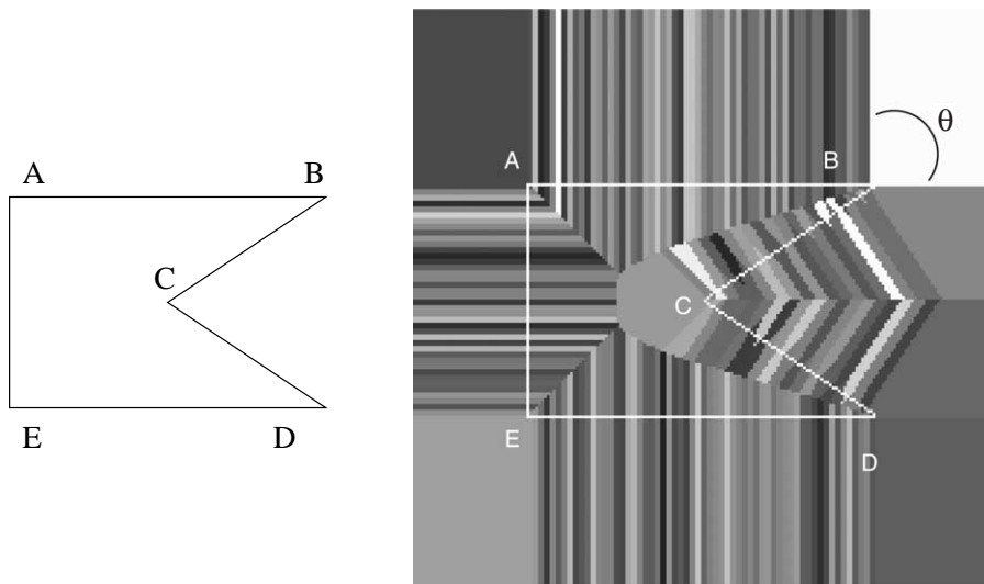
Fig. 1. A shape (left), the internal and external influence areas of its convex (A, B, D, and E) and concave (C) points, and an aperture angle \theta at point B (right).
