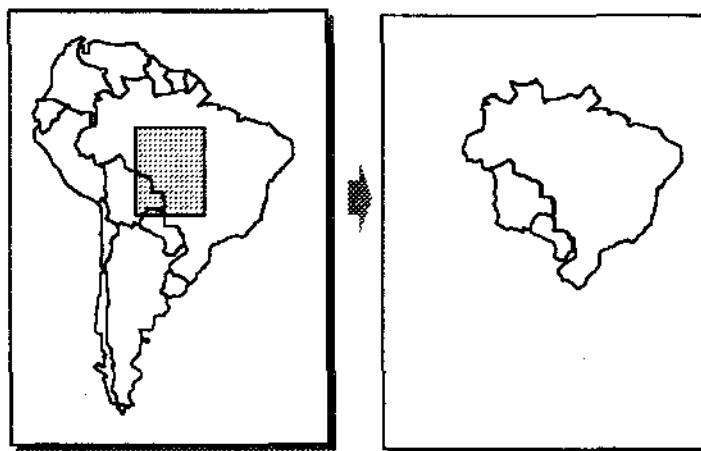
Fig. 4.2 - Windowing
