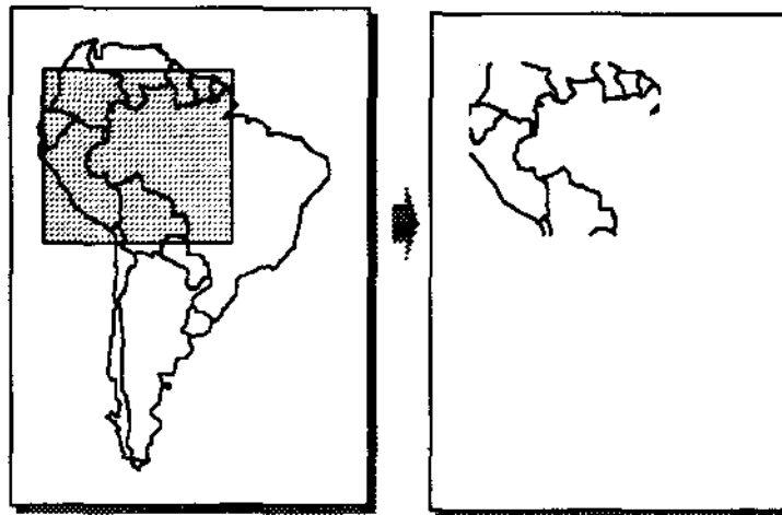
Fig. 4.3 - Clipping
