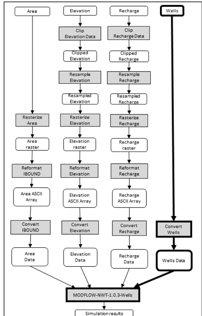
Figure 3. A workflow variant W 3 derived from W 2 is created in Scenario S3 after adding well data, which requires adding the necessary data conversion steps and also changing the MODFLOW component to have an additional input for well data. The new and modified components are shown with a thicker outline.
